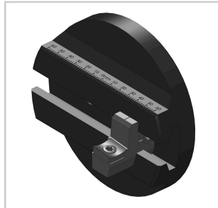
Sliding adjustment of tool Holder (30 or 45° bevel angle)
